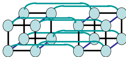
Direct Tree
