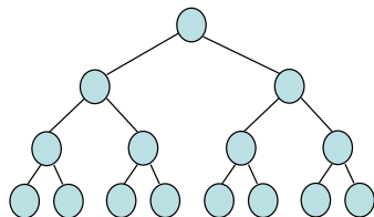
Direct Tree
