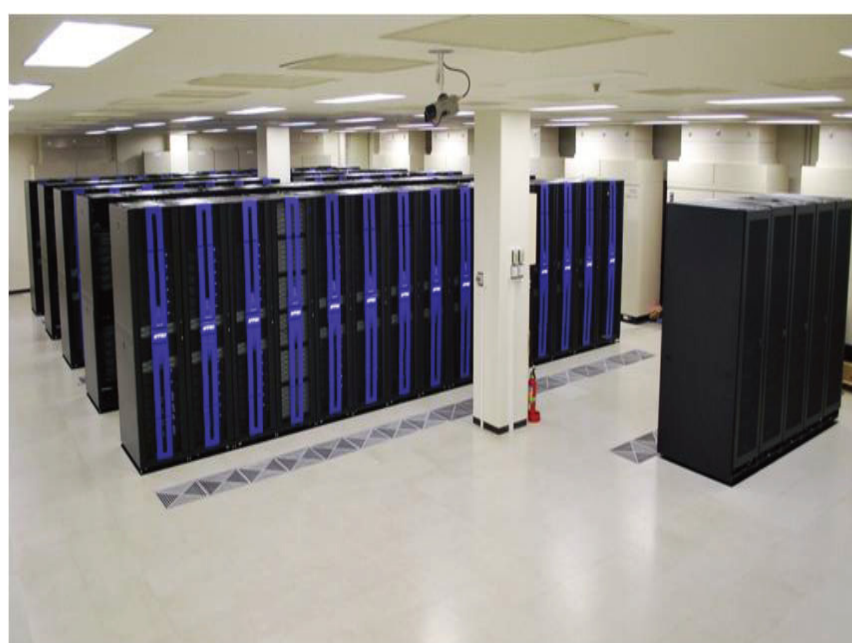
T2K-Tsukuba
